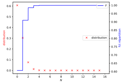
(a) \lambda = \frac{1}{2}
